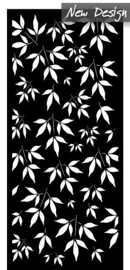
Canopy ≈ 21% Vis
