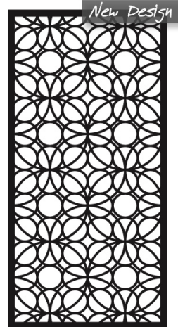
Rings ≈ 54% Vis
