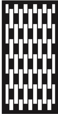
Chainmail ≈ 42% Vis
