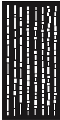
Birch ≈ 19% Vis
